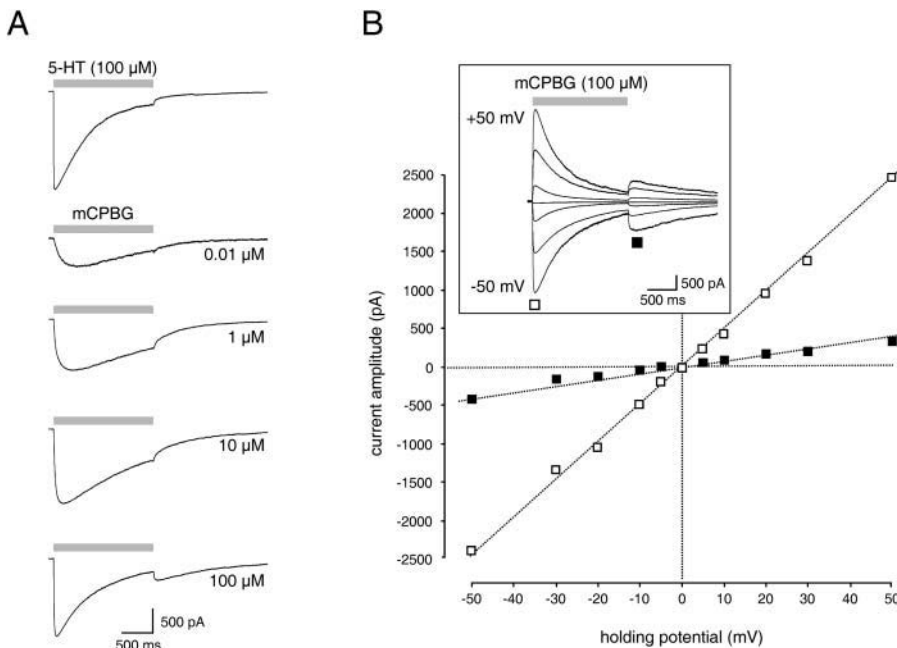
FIGURE 10 Application of mCPBG to cells carrying heteromeric 5-HT 3AB receptors. (A) 5-HT (100 μM) induced an inward current without tail current ( top ). mCPBG also induced inward currents. In contrast to 5-HT, the withdrawal of mCPBG (100 μM) induced a tail current ( bottom ). (B) The mCPBG-induced responses did not show any rectification.
