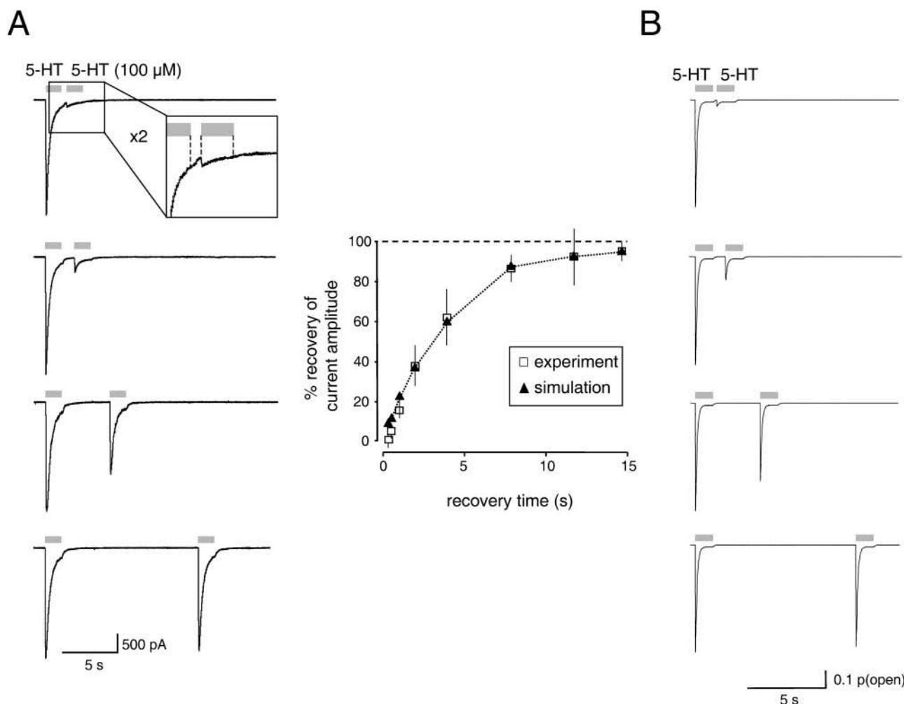
FIGURE 6 Kinetics of 5-HT 3AB receptor resensitization. Repetitive pulses (gray bars) of 5-HT (100 μM) were applied. (A) Current traces from a representative cell. (B) Simulated currents (5-HT 3AB receptor model, see Fig. 2 E). Recovery of the response to >50% (>95%) required 3 s (12 s, mean ± SD, n = 5). After shorter intervals between the agonist pulses, a small current with kinetics similar to those of the initial response was induced by the second pulse (see also inset). This effect is reconciled with classical receptor desensitization and was also predicted by the model.
