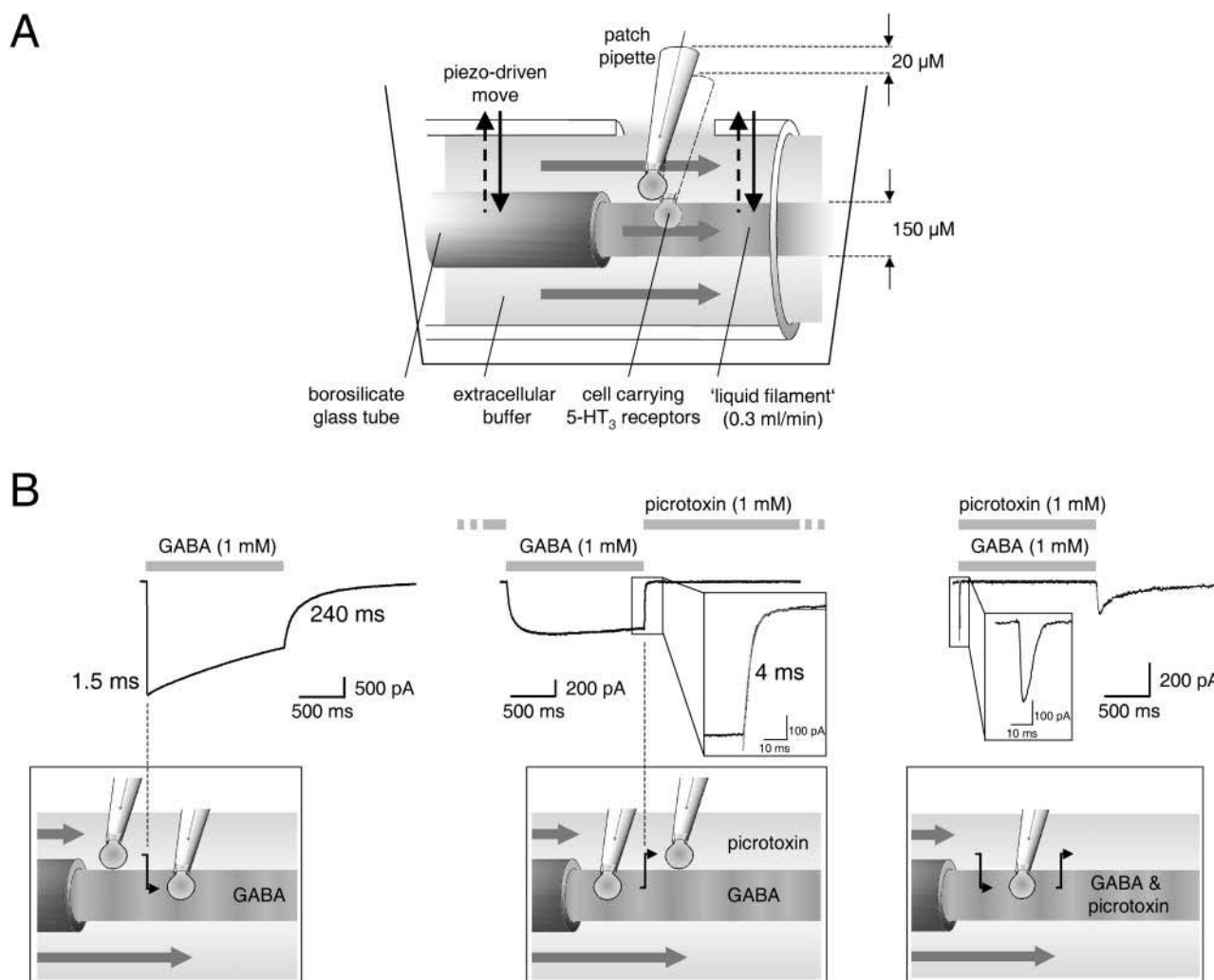
FIGURE 1 (A) The “fast-switch” system. To mimic the kinetics of synaptic release, a system for rapid exchange of solutions was used. The “liquid filament” consists of extracellular solution containing the agonist. Upon piezo-crystal activation, it shifts upward by 20 \mu\text{m} and the whole-cell patch carrying the 5-HT 3 receptors is immersed. Upon piezo inactivation, the liquid filament shifts downward to the resting position. This device allows for a complete exchange of solutions in the vicinity of the cell within 1–5 ms. (B) The time required for complete application of the liquid filament is, at most, 1.5 ms: activation of GABA A receptors by 1 mM GABA reveals a rise time of the GABA-induced current of 1.5 ms ( left ). The time required for withdrawal of the liquid filament is, at most, 4 ms: the piezo-driven switch from the liquid filament (GABA solution) to buffer containing the noncompetitive GABA A receptor blocker picrotoxin (1 mM) considerably accelerates the decay of the GABA response, revealing a time constant of 4 ms ( mid ). When GABA and picrotoxin are co-applied, the GABA response is rapidly reduced. On rapid withdrawal of the liquid filament, the unblocking of picrotoxin evokes a tail current ( right ).
