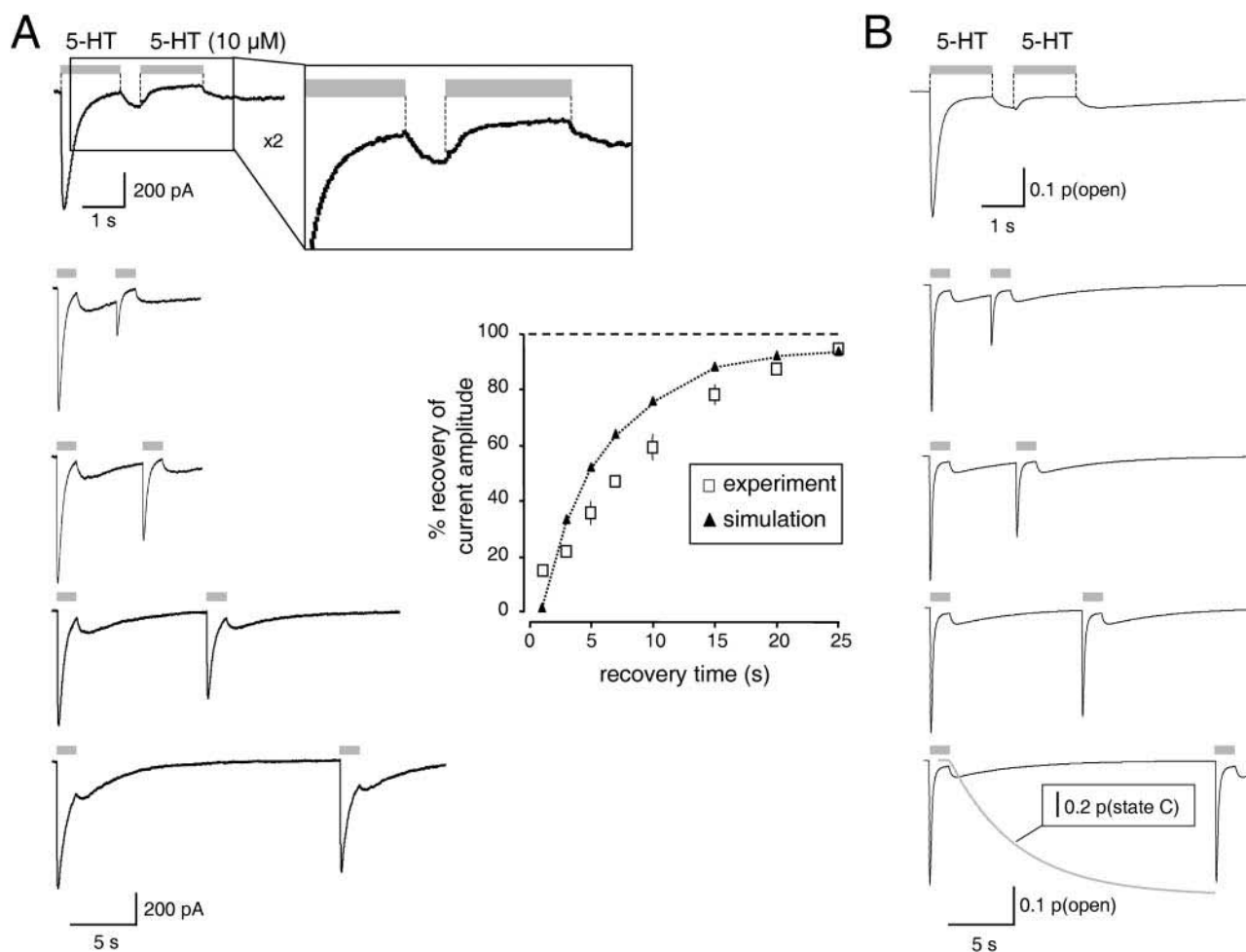
FIGURE 5 Kinetics of 5-HT 3A receptor resensitization. Repetitive pulses (gray bars) of 5-HT (10 \mu M) were applied. (A) Current traces from a representative cell. (B) Simulated currents (model provided in Fig. 2 B). Recovery of the response to >50% (>95%) required 7 s (25 s, mean \pm SD, n = 3 ). An interval of 0.5 s between the two agonist pulses resulted in an overlap of the second pulse and the tail current (A, top, inset) resulting in a current decay within the tail current. This effect, which is reconciled with an agonist-induced open-channel block, was also predicted by the model (B, top).
